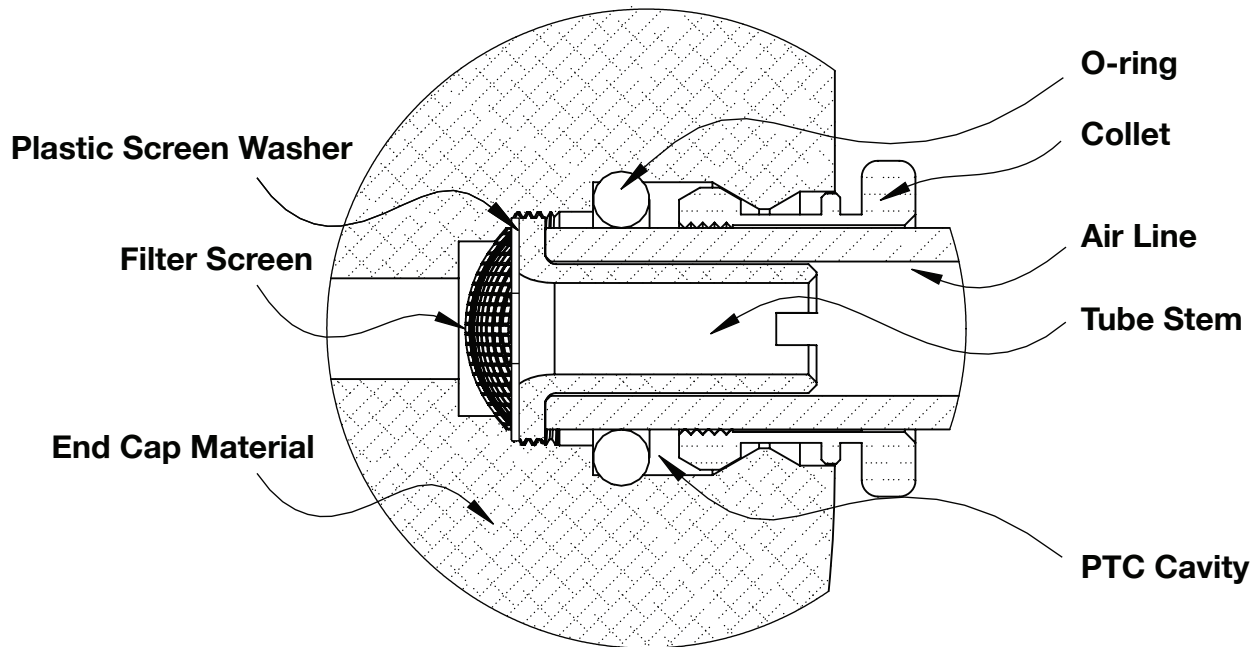
Figure 11: PTC diagram
