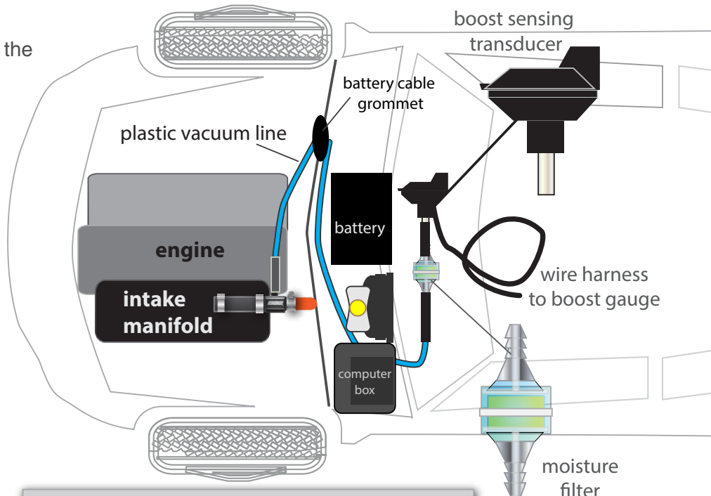
Vacuum Routing Map Audi B7 A4 Vacuum/Boost Gauge
