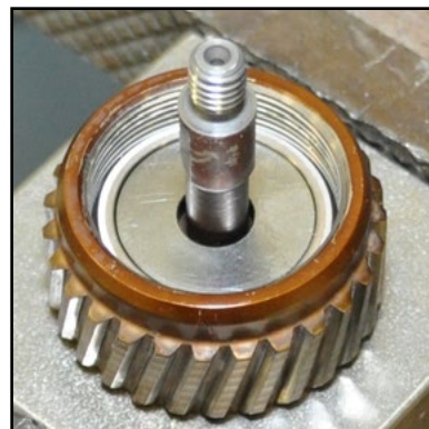
Install the other end washer
