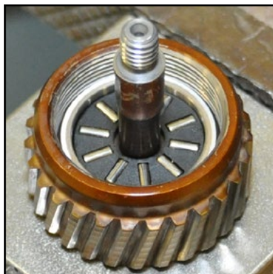
Install the other bearing
