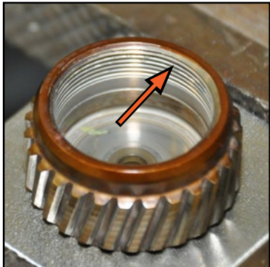
Clean all remaining thread locking compound out of the transfer gear threads
