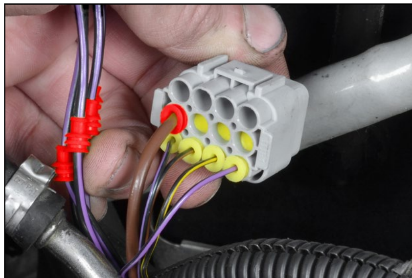
Locking tabs
