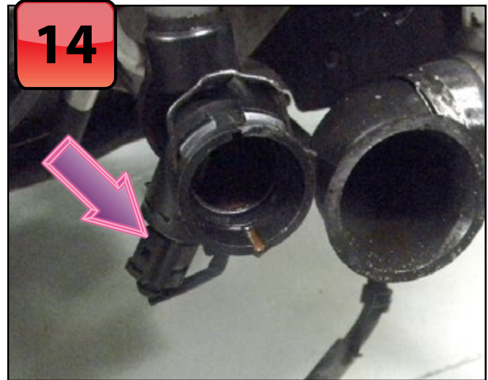
The lower radiator hose and air inlet hose for the charge air cooler must also be disconnected. There is no radiator drain plug. The coolant sensor may be disconnected and unscrewed to drain coolant—or just disconnect the lower radiator hose for the express drain feature!
