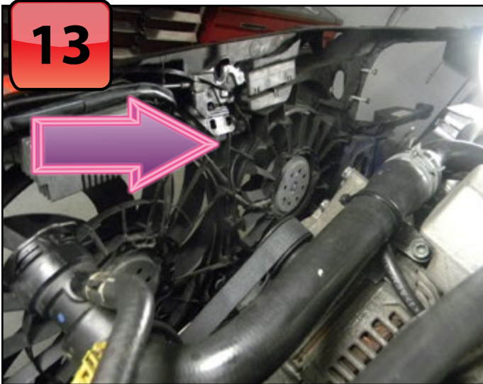
Don't forget to disconnect the hood latch sensor wire. It is hidden on the backside of the radiator header, between the fans. It's easy to miss. The wire snakes down to a connector near the bottom of the radiator support.
