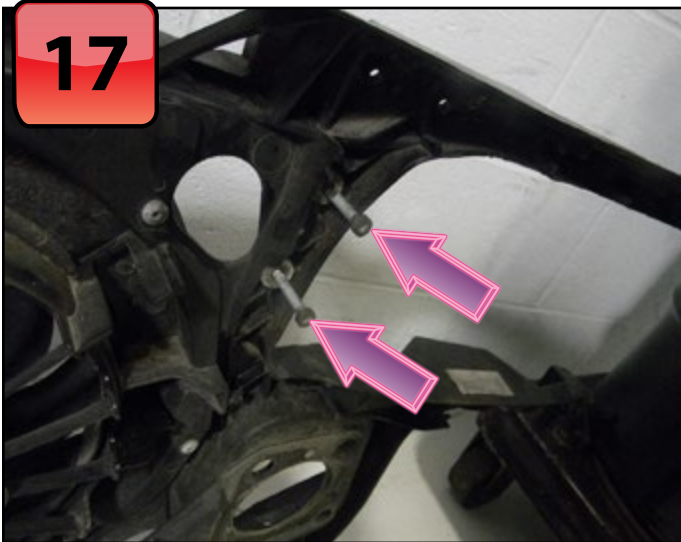
The crash sensors bolt to the radiator support with two Allen head screws. Our photo shows the bolt locations on the right side with the sensor already removed.
