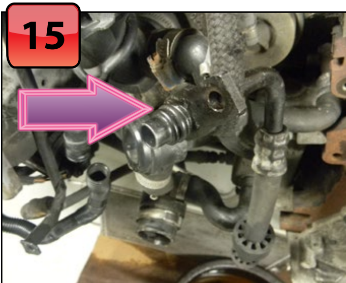
Check the transmission cooler line o-rings for damage. Note the location of the bolt hole for the attachment bracket.
